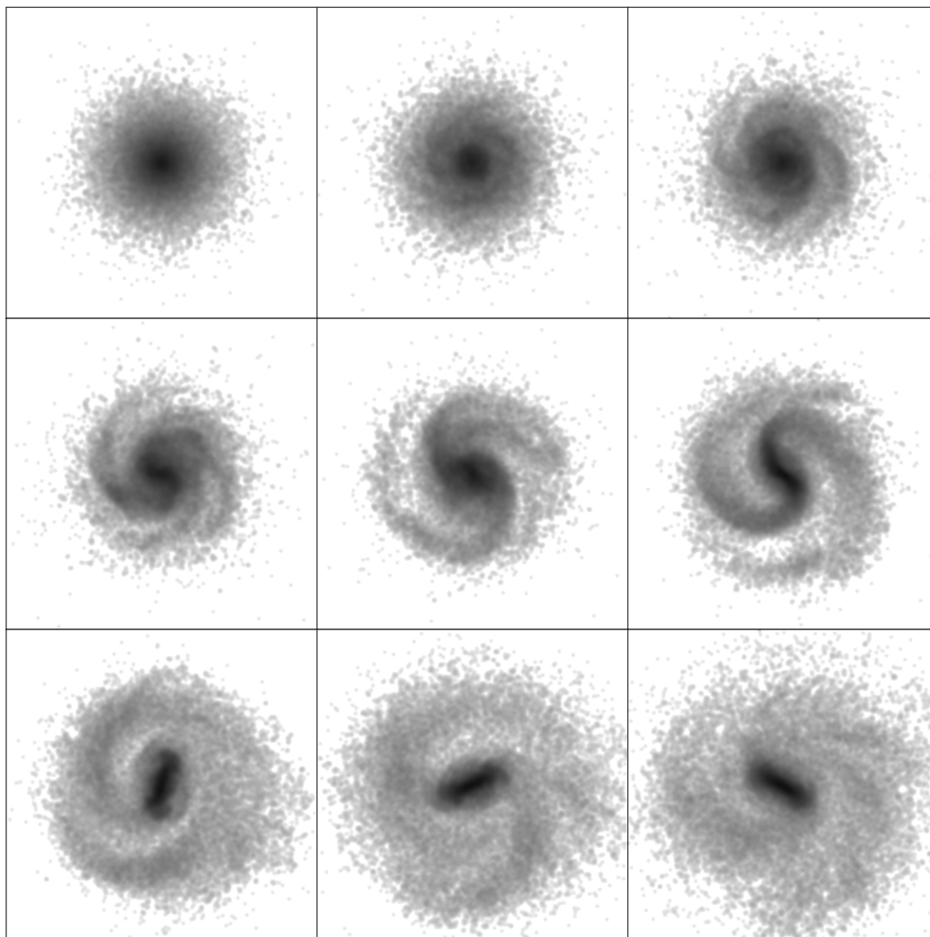
Figure 19.1: Bar instability in a model disk galaxy. This model is similar to the one shown in Fig. 18.2, but here the disk comprises 75% of the total
