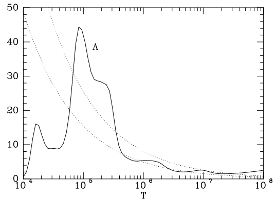
FIG. 1.— Full curve: the cooling coefficient \Lambda(T) for a plasma with 0.4 of solar abundances. Dashed curves: curves proportional to T^{-1/2} that intersect the full curve at T = 3.5 and 4.5 \times 10^5 K.
