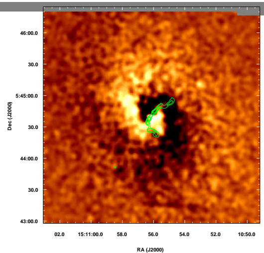
FIG. 3.— Residual image of the central 275 kpc of Abell 2029. The image was made by subtracting a smooth elliptical model from the Gaussian ( \sigma = 2'' ) smoothed Chandra data. Contours show the 1.4 GHz radio emission of PKS 1508+059 from Taylor, Barton, & Ge (1994). The large spiral X-ray excess may be the result of stripping of gas from an infalling cold cloud that had an initial non-zero angular momentum orbit. The linear feature seen 1'5 south of the cluster core is an absorption region associated with the disk of a foreground edge-on spiral galaxy.
