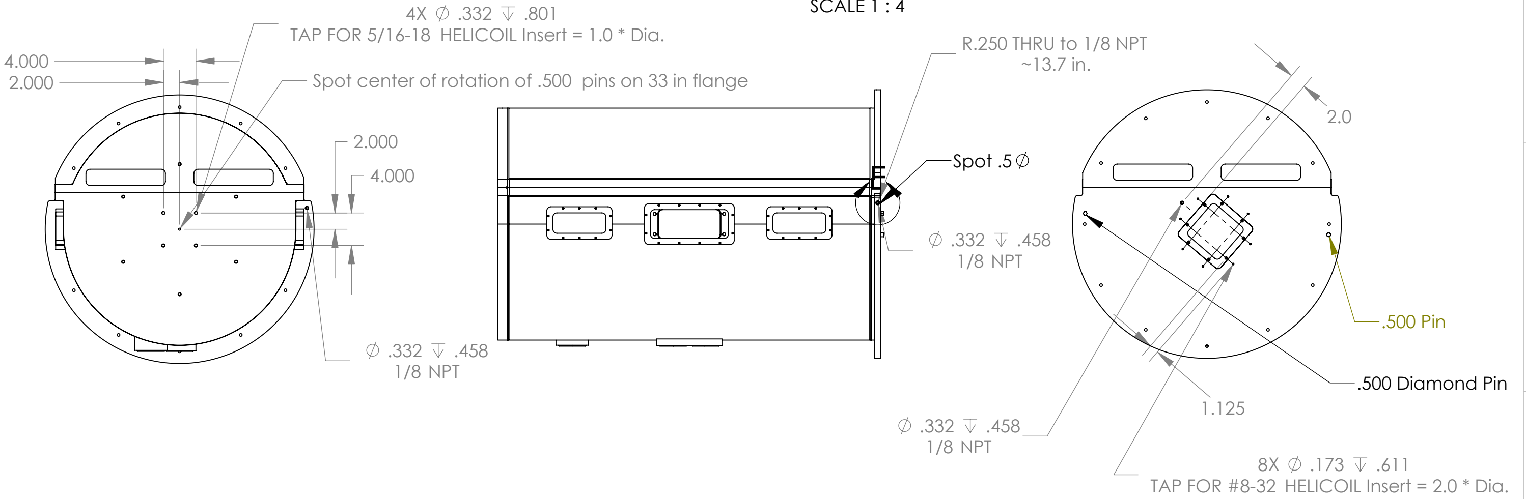
DETAIL E SCALE 1 : 4
