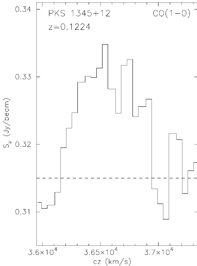
Fig. 2.—Extracted CO (1 → 0) spectrum of PKS 1345+12. The spectrum is smoothed with a \sim 80 km s ^{-1} filter and sampling of 40 km s ^{-1} intervals ( S_{\text{ms}} \sim 0.005 Jy).
