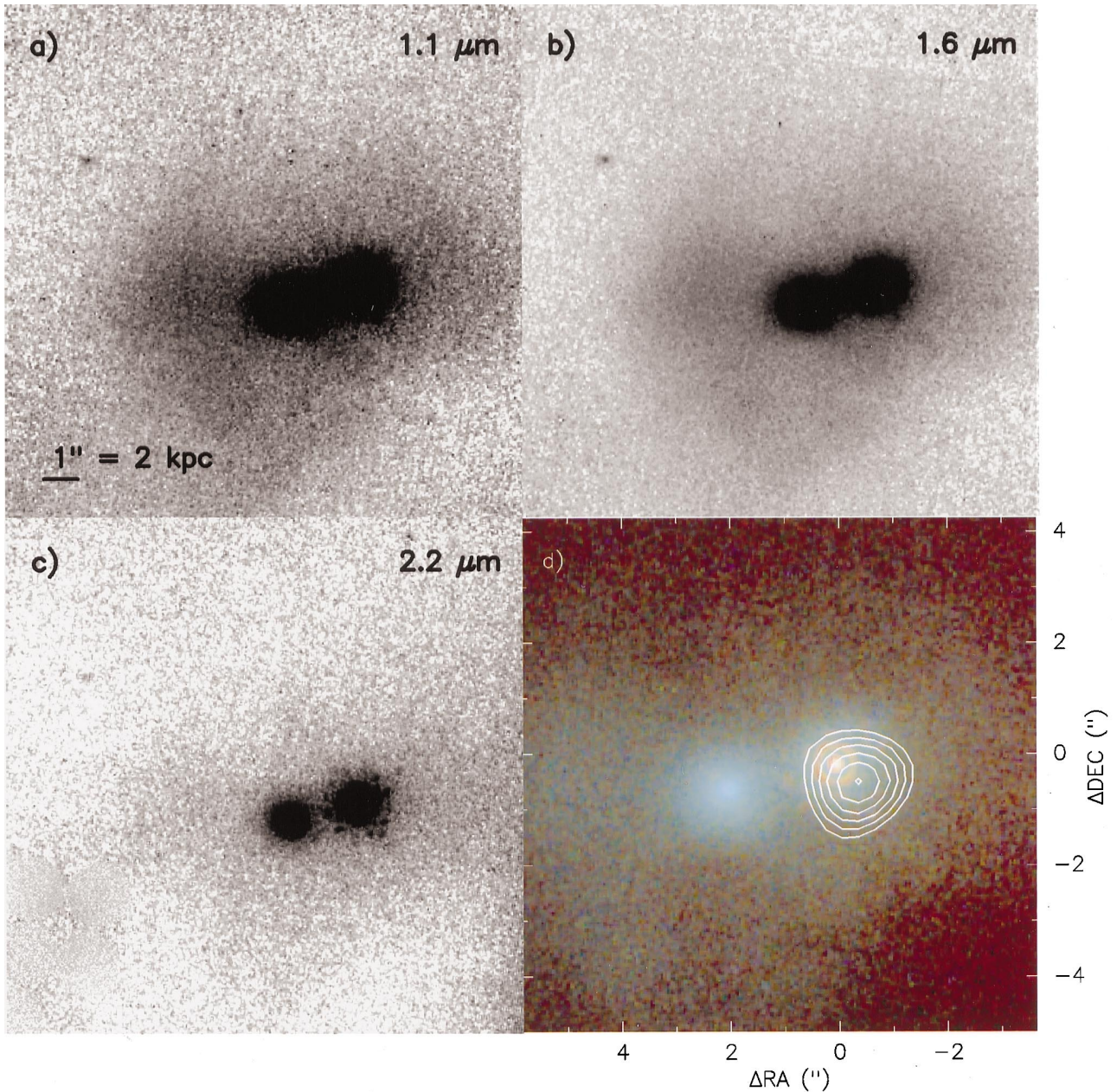
FIG. 1.—(a–c) HST NICMOS 1.1, 1.6, and 2.2 \mu\text{m} images of PKS 1345+12. The images have peak intensities of 7.5, 11, and 29 \mu\text{Jy} for the 1.1, 1.6, and 2.2 \mu\text{m} images, respectively. The speckle pattern surrounding PKS 1345+12NW at 2.2 \mu\text{m} is a point-spread function artifact. (d) Continuum-subtracted CO (1 \rightarrow 0) emission superposed on the false-color NICMOS image. The NICMOS data are displayed with blue as 1.1 \mu\text{m} , green as 1.6 \mu\text{m} , and red as 2.2 \mu\text{m} . The CO data are plotted as 50%, 60%, 70%, 80%, 90%, and 99%, where 50% corresponds to 3.9 \sigma rms and 100% corresponds to a peak flux of 0.0339 Jy \text{beam}^{-1} . The CO emission is unresolved, with a beam FWHM of 2.46 \times 1.95 at a position angle of -70^\circ 5 .
