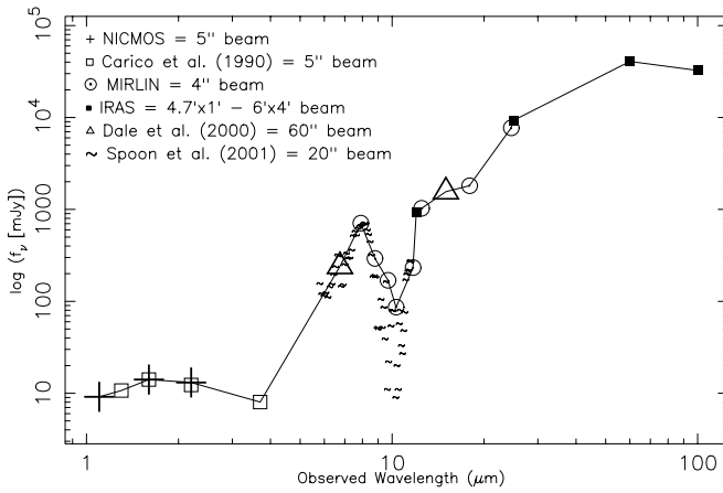
FIG. 4.—Spectral energy distribution of NGC 4418 based on broadband measurements. The solid line is a fit to the broadband data. Note the agreement between the broadband data and the ISO-PHT-S data.
