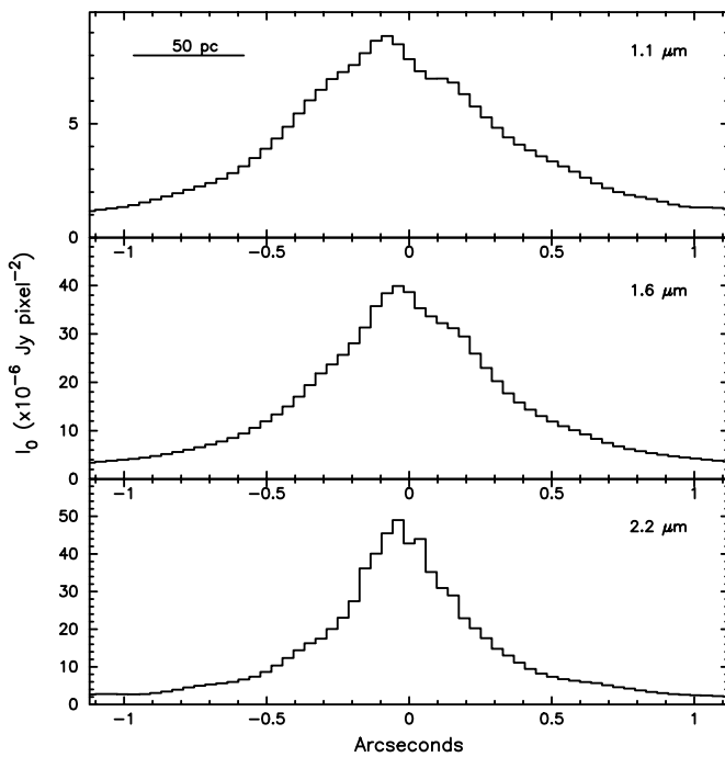
FIG. 3.—Intensity-profile plots of the nuclear structure. The profiles, which have a width of 0''.0386 , have been extracted from the deconvolved/Gaussian-smoothed images.
