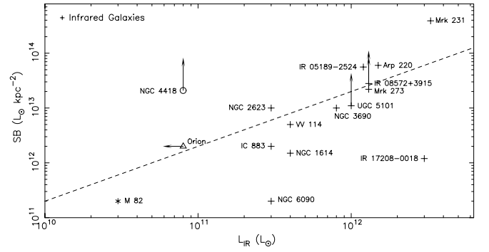
FIG. 5.—Plot of the infrared surface brightness vs. infrared luminosity for NGC 4418 and a sample of objects discussed in Soifer et al. (2000, 2001). The dashed curve is an example of an isosurface area curve; all such curves on Fig. 5 are parallel to the dashed curve.
