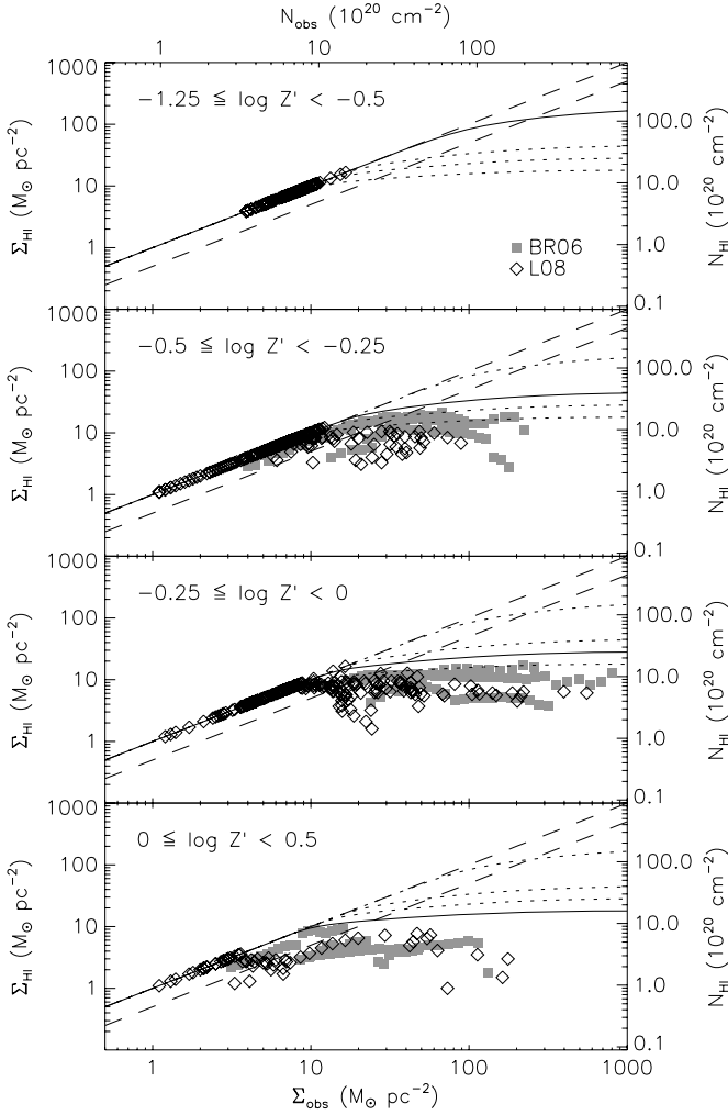
Figure 4. H I column density \Sigma_{\text{HI}} vs. total column density \Sigma for galaxies in metallicity bins -1.25 < \log Z' < -0.5 , -0.5 < \log Z' < -0.25 , -0.25 < \log Z' < 0 , and 0 < \log Z' < 0.5 , as indicated. In each panel we plot the values of \Sigma_{\text{HI}} and \Sigma from the samples of BR06 (squares) and L08 (diamonds) and show our model predictions of \Sigma_{\text{HI}} as a function of \Sigma for \log Z' = -0.5 , -0.25 , 0 , and 0.5 (lines, highest to lowest). The curve for the value of \log Z' equal to the maximum \log Z' for each bin, which should represent the upper envelope of the data, is shown as a solid line. The rest are shown as dotted lines. The four lines are the same in each panel. To maximize readability we omit the error bars on the data points. The parallel slanted dashed lines, \Sigma_{\text{HI}} = \Sigma_{\text{obs}}/2 and \Sigma_{\text{HI}} = \Sigma_{\text{obs}} , show the range of values of \Sigma_{\text{HI}} for which our predictions should be treated as upper limits for the reasons discussed in Section 3.3. Parts of our model curves above the \Sigma_{\text{HI}} = \Sigma_{\text{obs}}/2 line could be as high as the \Sigma_{\text{HI}} = \Sigma_{\text{obs}} line.
