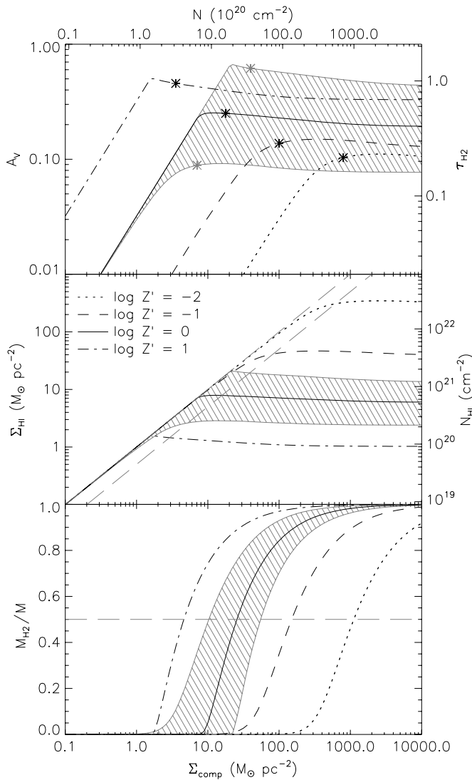
Figure 2. Visual extinction A_V (top panel), H I column density \Sigma_{\text{HI}} (middle panel), and H 2 fraction M_{\text{H}_2}/M (bottom panel) in finite cloud complexes, as a function of complex mass column density \Sigma_{\text{comp}} (or number column density N ). In each panel the curves shown are for metallicities Z' running from 10^{-2} – 10^1 , as indicated. The hatched regions centered on the Z' = 0 curve indicate the range of models with \phi_{\text{CNM}} = 1 - 10 , while all other curves are for our fiducial value \phi_{\text{CNM}} = 3 . In the top panel, the asterisks on the curves indicate the value of \Sigma_{\text{comp}} for which the molecular fraction falls to 1/2. The curves to the left of this point should be regarded as lower limits on the visual extinction to the molecular region. In the middle panel the two parallel dashed lines indicate ratios of M_{\text{HI}}/M = 1/2 and 1. Since values of M_{\text{HI}} below 1/2 are lower limits, once our models curves cross the lower of these lines, their true solution could be anywhere between them. Similarly, the dashed line in the bottom panel corresponds to M_{\text{H}_2}/M = 1/2 , and when the model curves fall below this they should be treated as upper limits.
