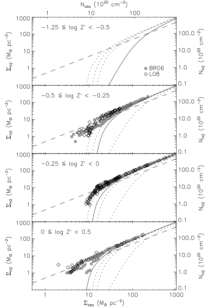
Figure 5. Same as Figure 4, except that we show H 2 rather than H I column densities. For clarity we do not show nondetections. Note that N_{\text{H}_2} is the column density of H nuclei in molecular form, which is twice the column density of H 2 molecules. The slanted dashed line is \Sigma_{\text{H}_2} = \Sigma_{\text{obs}}/2 ; as discussed in Section 3.3, above this line our model curves may be taken as predictions, while below it they should be taken as upper limits.
