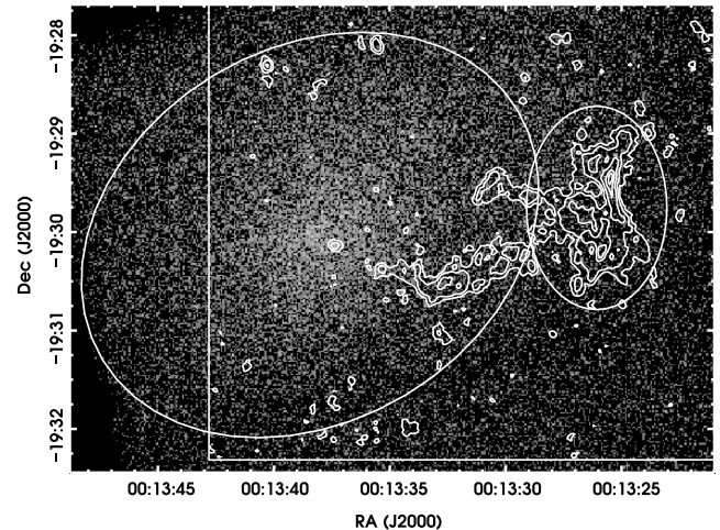
FIG. 6.—Raw Chandra X-ray image ( 0.3 - 10 keV) of Abell 13 encompassing the cluster center and radio relic positions. Overlaid are the radio contours of Slee et al. (2001). The straight lines mark the coverage of the VLA data compared to the Chandra data. The large ellipse marks the region of the data used to determine the spectral model of the full cluster emission (§ 3.1). The smaller ellipse on the right marks the region of the data used to measure the spectrum of the X-ray gas coincident with the radio relic (§ 3.3). The region covered is 6.6' \times 4.7' .
