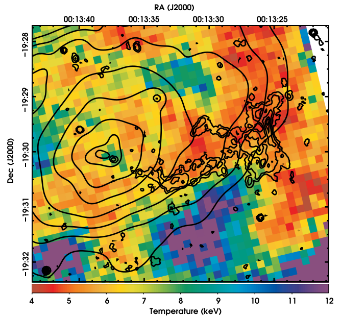
FIG. 8.—Temperature map of Abell 13. Red signifies regions of lower temperature, and purple of higher temperature. Overlaid are the X-ray and radio surface brightness contours. No cooling flow is detected. The coolest gas is to the west of the peak in the X-ray emission, and apparently associated with the radio relic.
