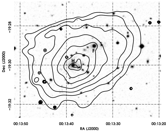
FIG. 2.—X-ray brightness contours (0.3–10 keV band, logarithmically spaced by a factor of \sqrt{2} ) overlaid on the DSS optical image scanned from a SERC-J survey plate taken in 1977 at the UK Schmidt telescope, Australia. The bright galaxies H and F from Slee et al. (2001) are labeled. The X-ray emission is centered near galaxy H. A knot of X-ray emission to the northwest of the cluster X-ray peak is consistent with the position of galaxy F. The steepness of the X-ray contours on the northern and eastern edges are artifacts of the CCD edge.
