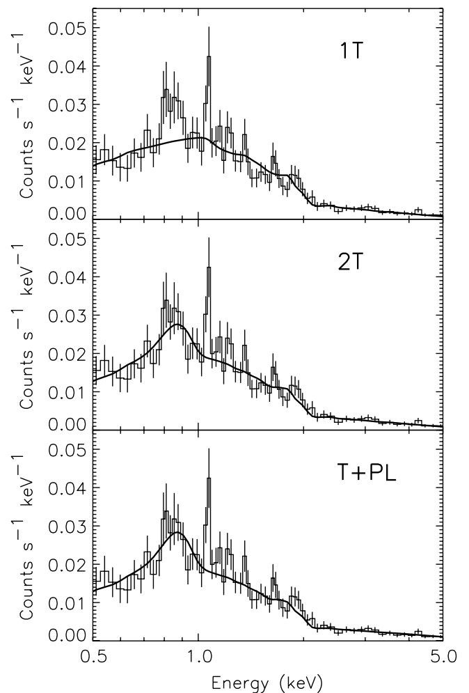
FIG. 9.—Count spectra of the X-ray emission associated with the radio relic, fit with different models. We have fit the spectrum with a single-temperature APEC model ( top ), two APEC models ( middle ), and a power law + APEC model ( bottom ). Note the soft excess at 0.8 keV in the single-temperature model ( top ) but not the other spectra. The peak at \sim 1.1 keV is too narrow to be astrophysical and is likely strengthened by binning. At other binnings, it is not as significant.
