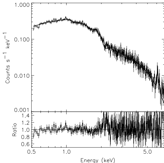
FIG. 7.— Top : Count spectrum of the X-ray emission from Abell 13 and the best-fit model. Bottom : Ratio of the data and best-fit model (data/model). The spectrum was extracted from a 2.5' \times 1.9' elliptical region encompassing the largest elliptical isophote contained fully on the S3 CCD. The best-fit model has a temperature kT = 6.0 \pm 0.3 keV and a metal abundance of 0.46 \pm 0.12 solar.
