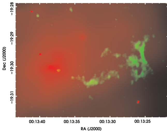
FIG. 3.—Radio image at 1.4 GHz (Slee et al. 2001) overlaid in green and the adaptively smoothed X-ray image of Abell 13 in red. North is up, and east is to the left. The region covered is 5.1' \times 3.8' . The radio image shows only emission detected at greater than 2.5\sigma as determined by Slee et al. (2001). The three compact red spots are X-ray point sources unrelated to the cluster.
