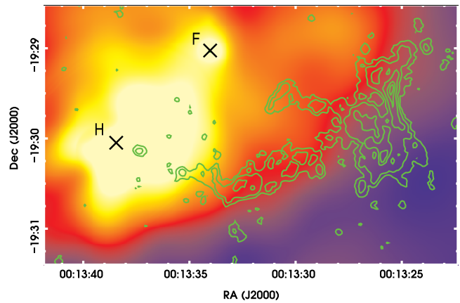
FIG. 4.—Residual X-ray emission from the cluster (color scale from blue = weak to white = strong) after partial subtraction of a smooth elliptical isophotal model for the entire cluster. The region shown here encompasses the radio relic and has a size of 4.6' \times 2.8' . The color scale was chosen to emphasize the outer regions of the cluster near the radio relic. Overlaid are the radio contours as given in Slee et al. (2001) with contour levels of 43, 86, 173, 303, and 389 \mu\text{Jy beam}^{-1} , which correspond to 2.5, 5, 10, 18, and 23\sigma . The two brightest galaxies H and F are indicated by the crosses. No excess or clearly associated deficit in X-ray emission is found coincident with the radio relic. Along the eastern tail of the radio emission there appears to be a sharp drop in the residual X-ray emission. However, this drop is not very strong in the total X-ray surface brightness. There is a strong gradient in the southern part of the cluster, but at a larger radius and farther south.
