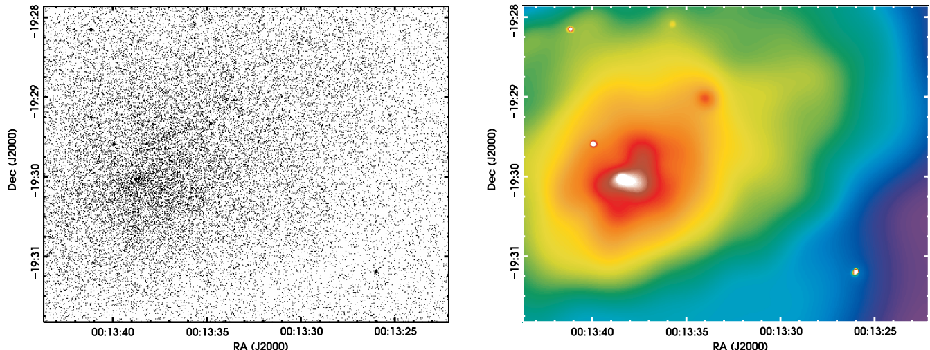
FIG. 1.— Left : Raw Chandra X-ray image (0.3–10 keV) of the 5' \times 4' region of Abell 13 encompassing the cluster center and radio relic positions. The image is uncorrected for exposure or background. North is up, and east is to the left. The image pixels are 0.492'' . Right : Adaptively smoothed Chandra X-ray image of the same region, corrected for background, exposure, and vignetting. Note the structure in the X-ray core as well as the knot of emission to the northwest of the core. In addition, the X-ray emission is extended to the northwest and west (toward the radio relic). The number of point sources is consistent with that expected from background sources.
