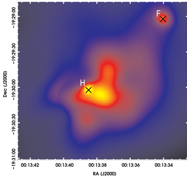
FIG. 5.—Residual emission from the center of Abell 13 after partial subtraction of a smooth elliptical isophotal model. The figure spans a region of 2.4' \times 2.2' . The color scale was chosen to emphasize the inner region of the cluster near galaxy H. North is up, and east is to the left. The bright region marked with a cross near the center coincides with galaxy H. Note the extension of emission to the west (in the direction of the radio relic) and the excess emission perpendicular to that direction. The cross at the top right corner marks the position of galaxy F.
