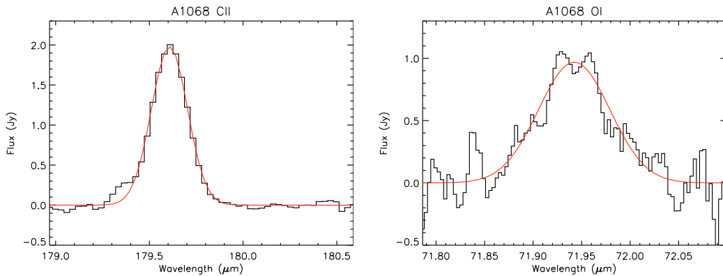
Fig. 1. Herschel -PACS spectra of [CII] and [OI] in A1068.
