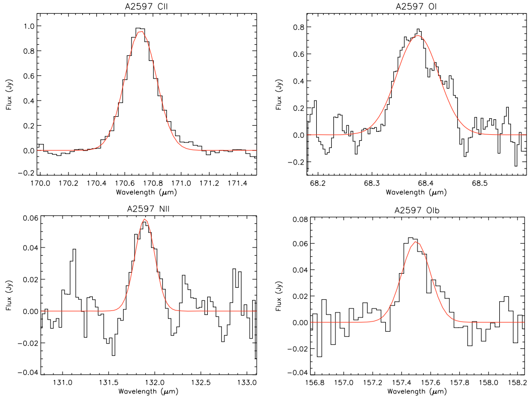
Fig. 2. Herschel -PACS spectra of [CII], [OI] (63 \mu\text{m} ), [NII] and [OIb] (145 \mu\text{m} ) in A2597.
