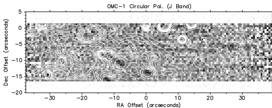
Figure 4. J -band circular polarization image of a small east–west strip in OMC-1 which stretches across the regions of high circular polarization that are seen in the other infrared bands. The circular polarization is scaled between -2 per cent (black) and +2 per cent (white). Offsets are west relative to the BN object.
