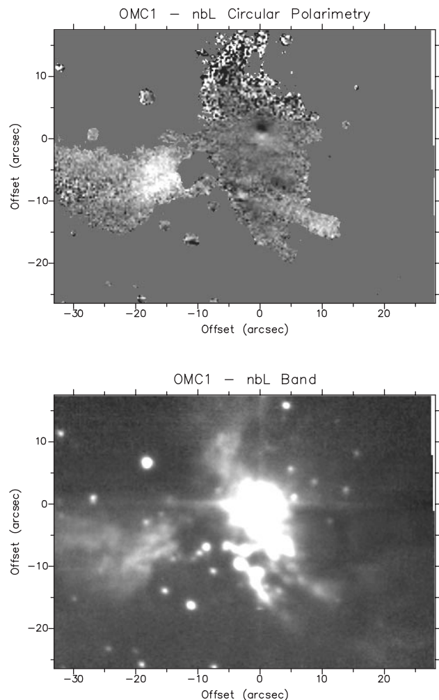
Figure 6. Narrow L -band (nb L ) imaging circular polarimetry of the OMC-1 region. The top panel shows the polarimetry scaled between -1 per cent (black) and +5 per cent (white). The observations have had low signal-to-noise ratio data masked out. The bottom panel shows the corresponding intensity distribution. Offsets are west from the BN object.
