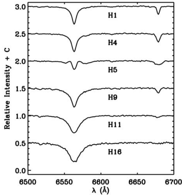
Figure 2. FOBOS red spectra of a representative sample of B stars in NGC 2169 showing the region of the H\alpha \lambda 6563 \text{ \AA} and He \text{ I } \lambda 6678 \text{ \AA} lines.
