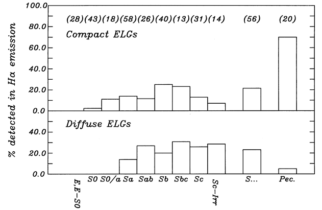
Figure 3. (Upper panel) The percentage detection of compact H \alpha + [N II] emission for galaxies in different Hubble type bins. (Lower panel) As upper panel, for diffuse emission. The total sample number for each bin is given in parentheses.
