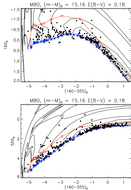
Fig. 2. (160, 160–555) and (555, 160–555) CMDs ( 555 \approx V ) for the BT cluster M80. The plots are based on data from Ferraro et al. (1998) and unpublished stellar models of Dorman. The lower line with *’s is the ZAHB; the upper line with \diamond ’s marks the points on the evolutionary tracks where models have reached 90% of their core He burning age.
